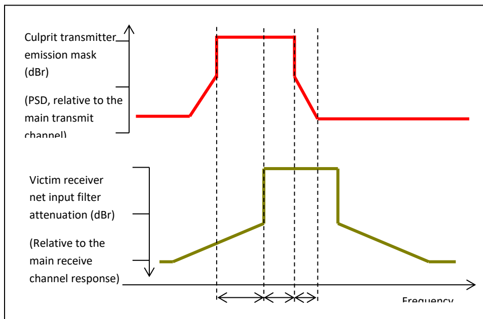
Figure 17: Example showing areas of three types of interference mechanism.
