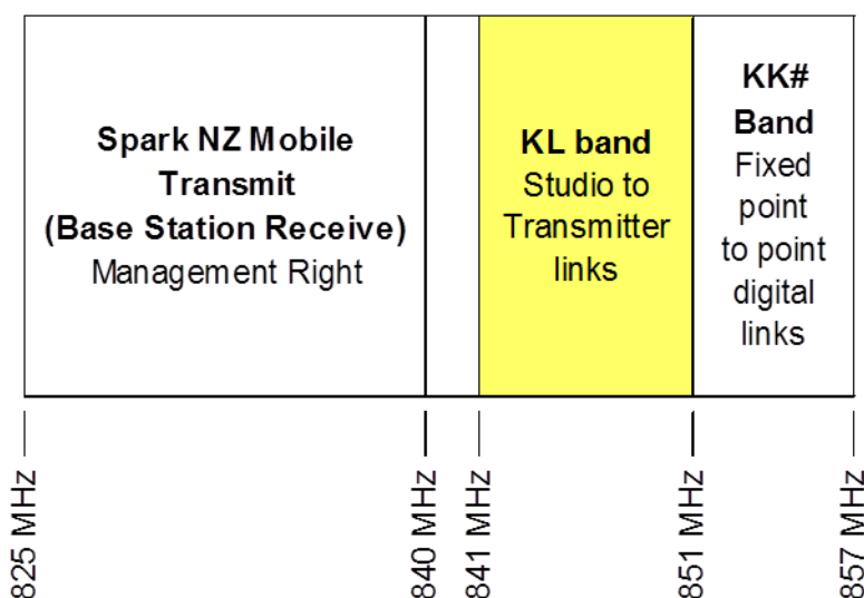
Figure 12: This is a chart of the KL band and the adjacent bands
