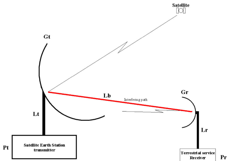
Figure 15: This shows a simplified interference scenario between a terrestrial service and a SES at a known azimuth/elevation angle when communicating with a geostationary satellite. It also shows losses and gains to be considered
